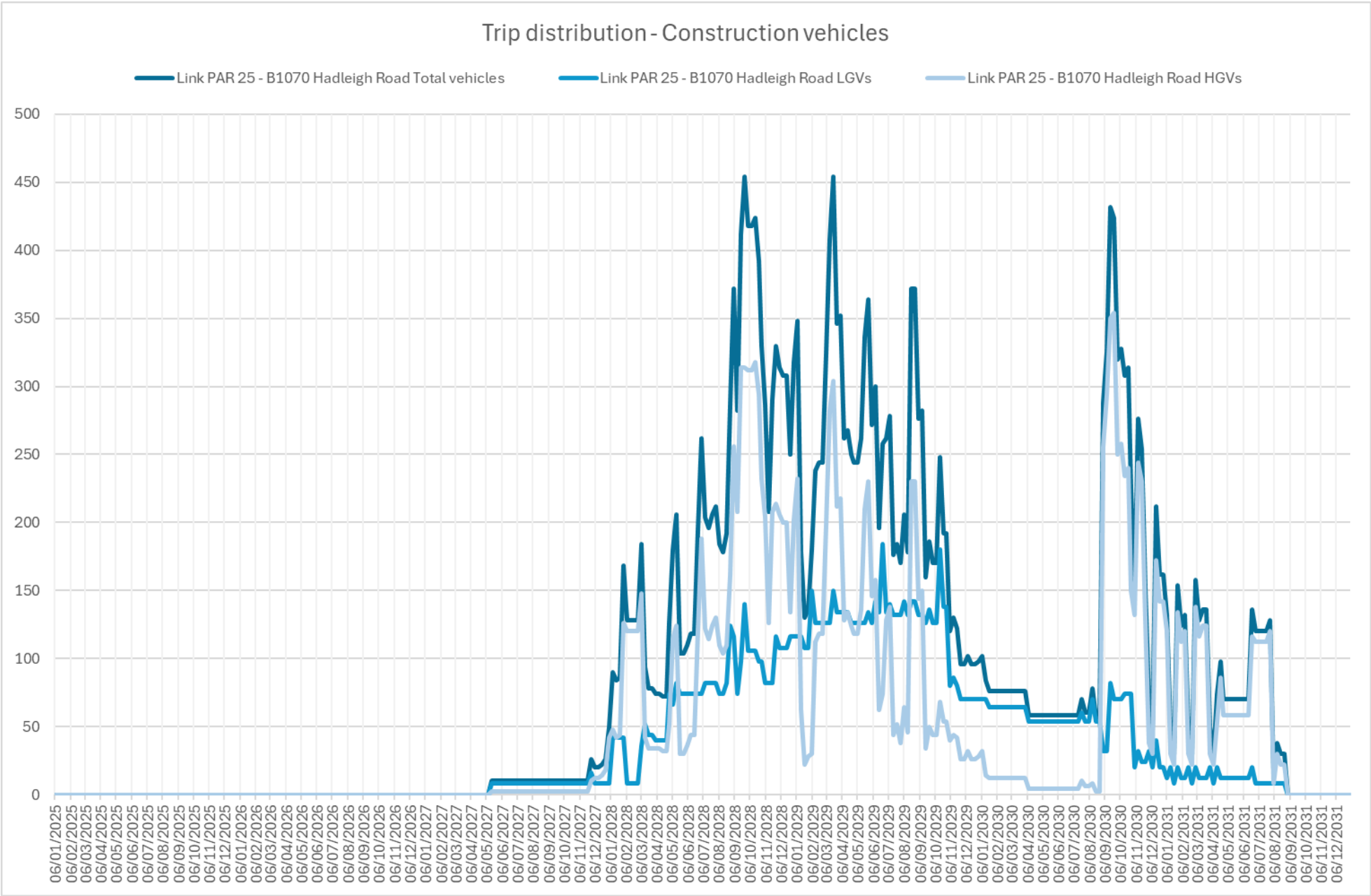
Image A16.4.25 Construction vehicles daily trip distribution of B1070 Hadleigh Road (Link PAR 25)
