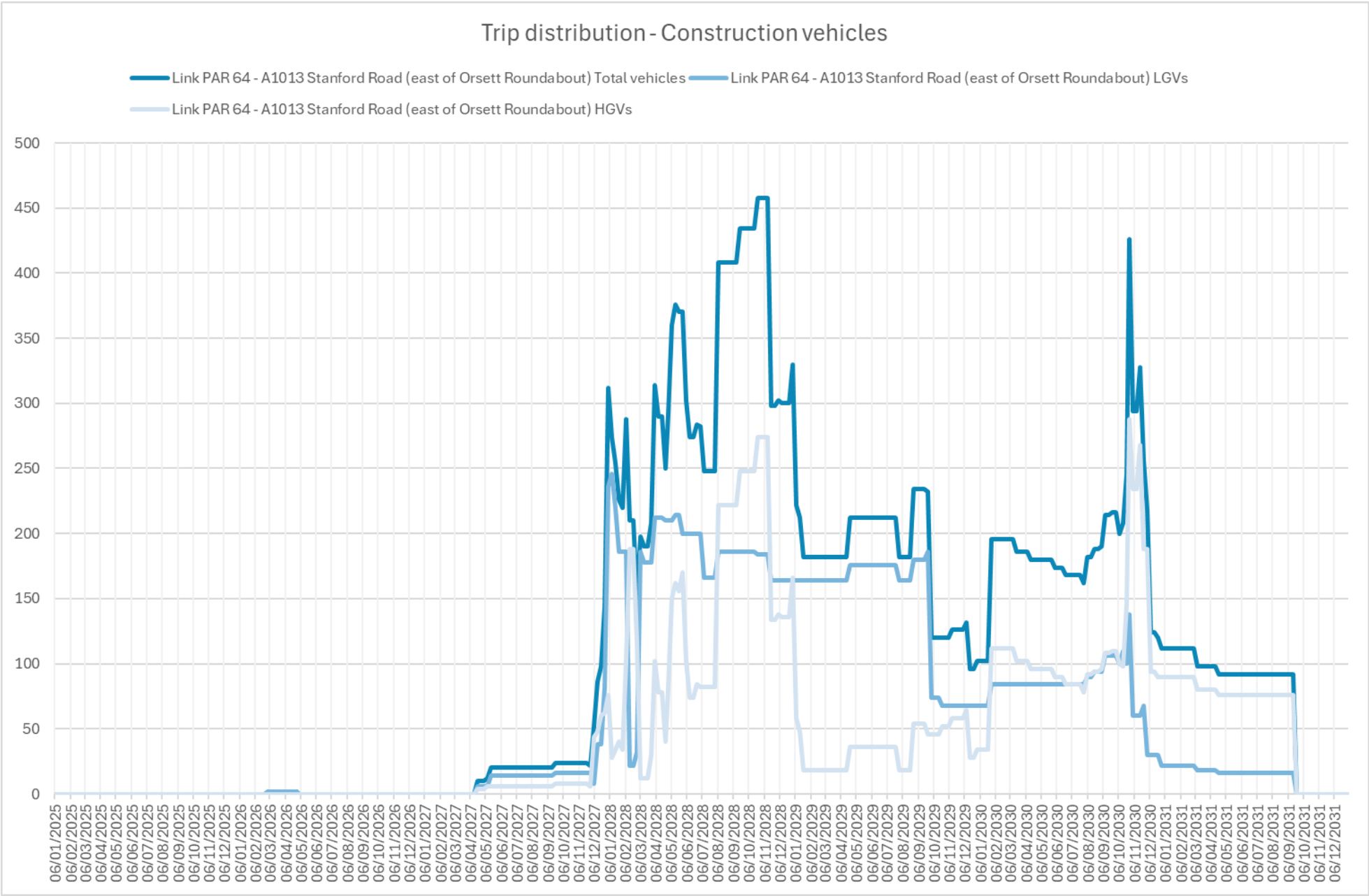
Image A16.4.64 Construction vehicles daily trip distribution of A1013 Stanford Road east of Orsett Cock Roundabout (Link PAR 64)
