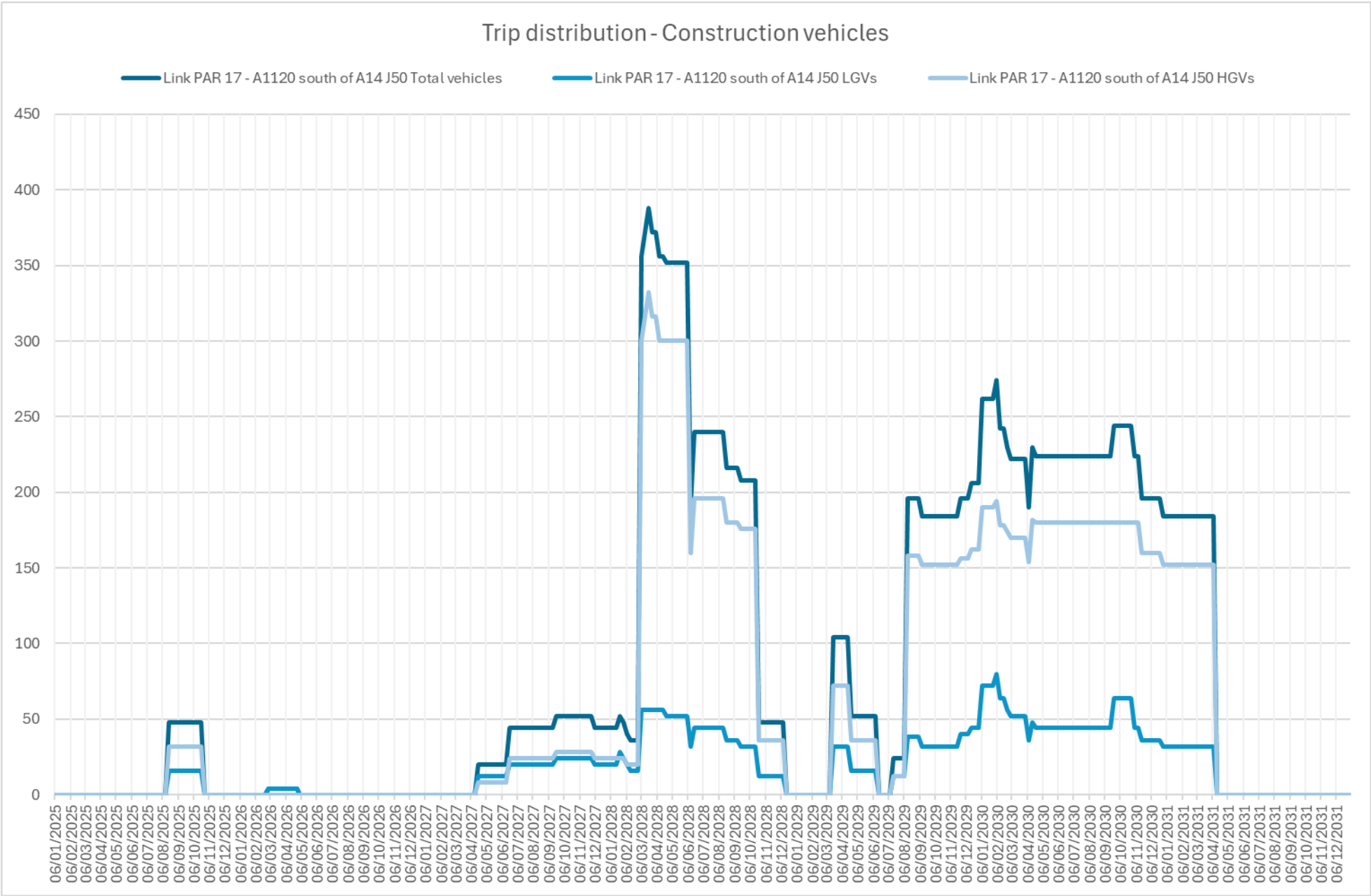
Image A16.4.17 Construction vehicles daily trip distribution of A1120 south of A14 J50 (Link PAR 17)
