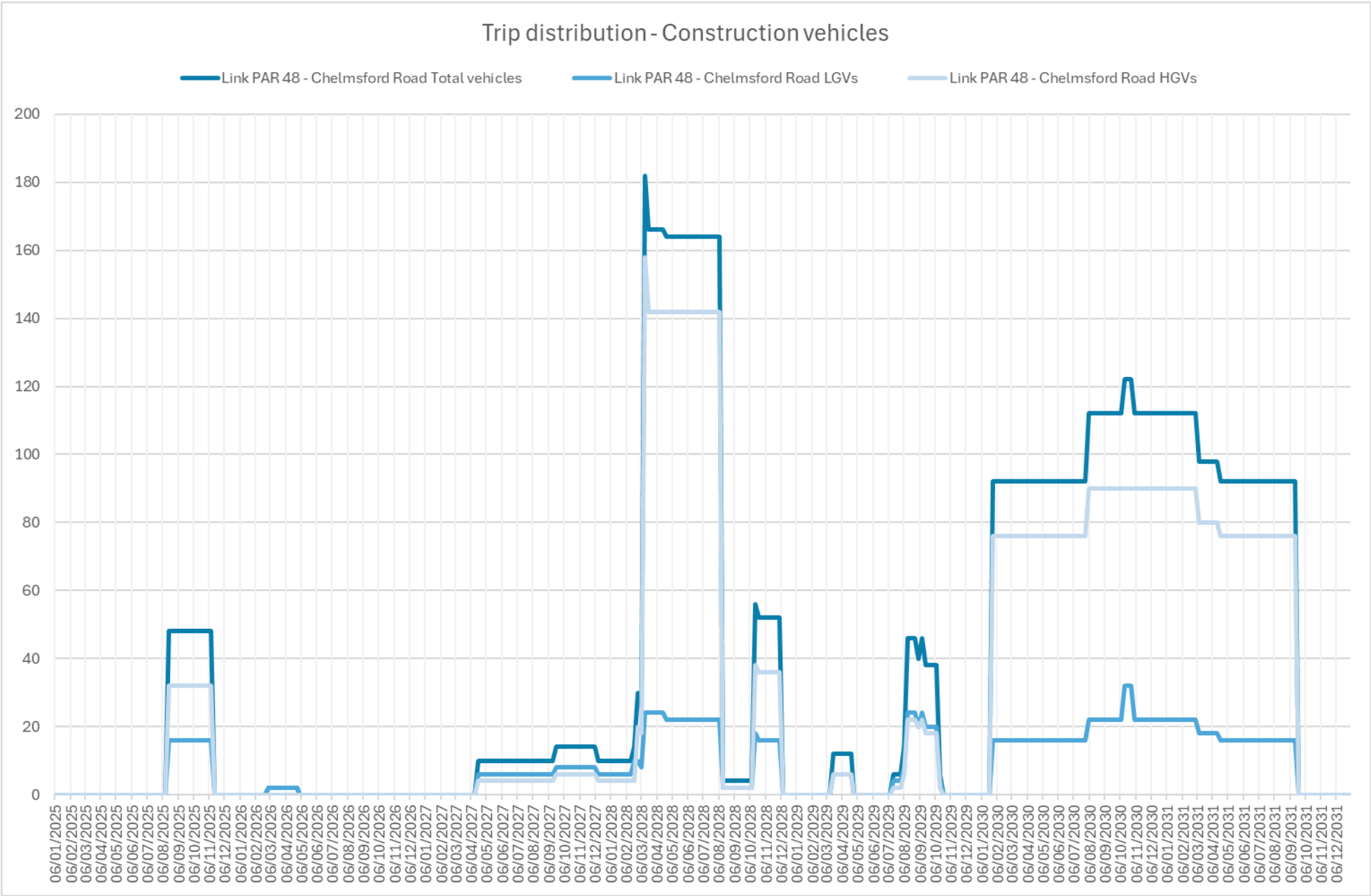
Image A16.4.48 Construction vehicles daily trip distribution of Chelmsford Road (Link PAR 48)
