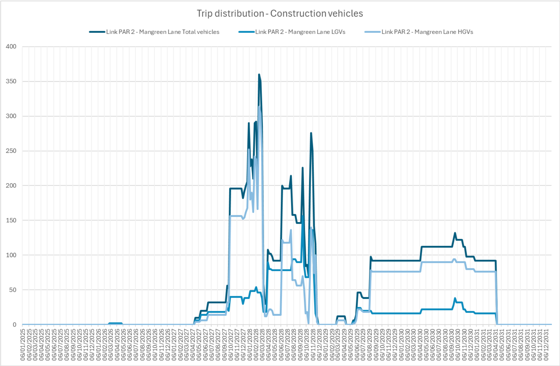
Image A16.4.2 Construction vehicles daily trip distribution of Mangreen Lane (Link PAR 2)
