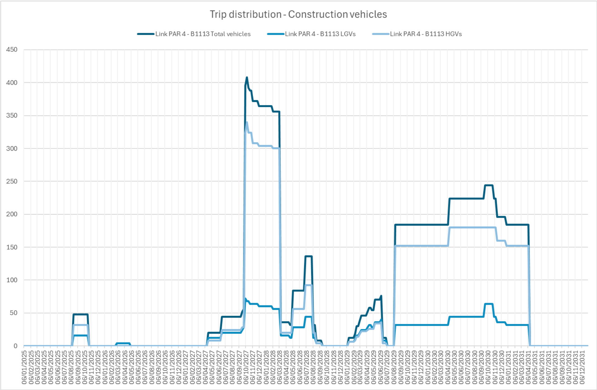
Image A16.4.4 Construction vehicles daily trip distribution of B1113 (Link PAR 4)
