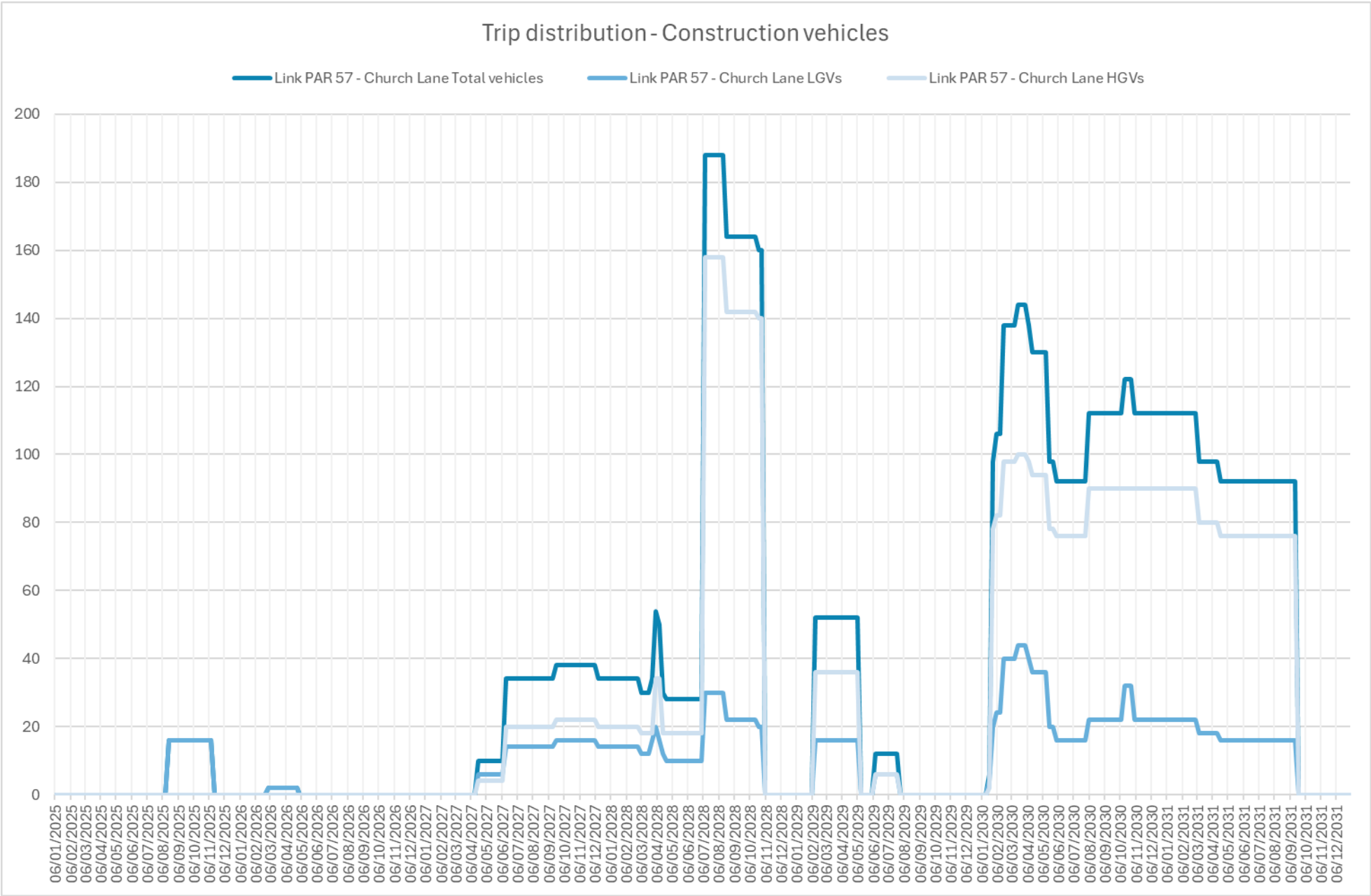
Image A16.4.57 Construction vehicles daily trip distribution of Church Lane (Link PAR 57)
