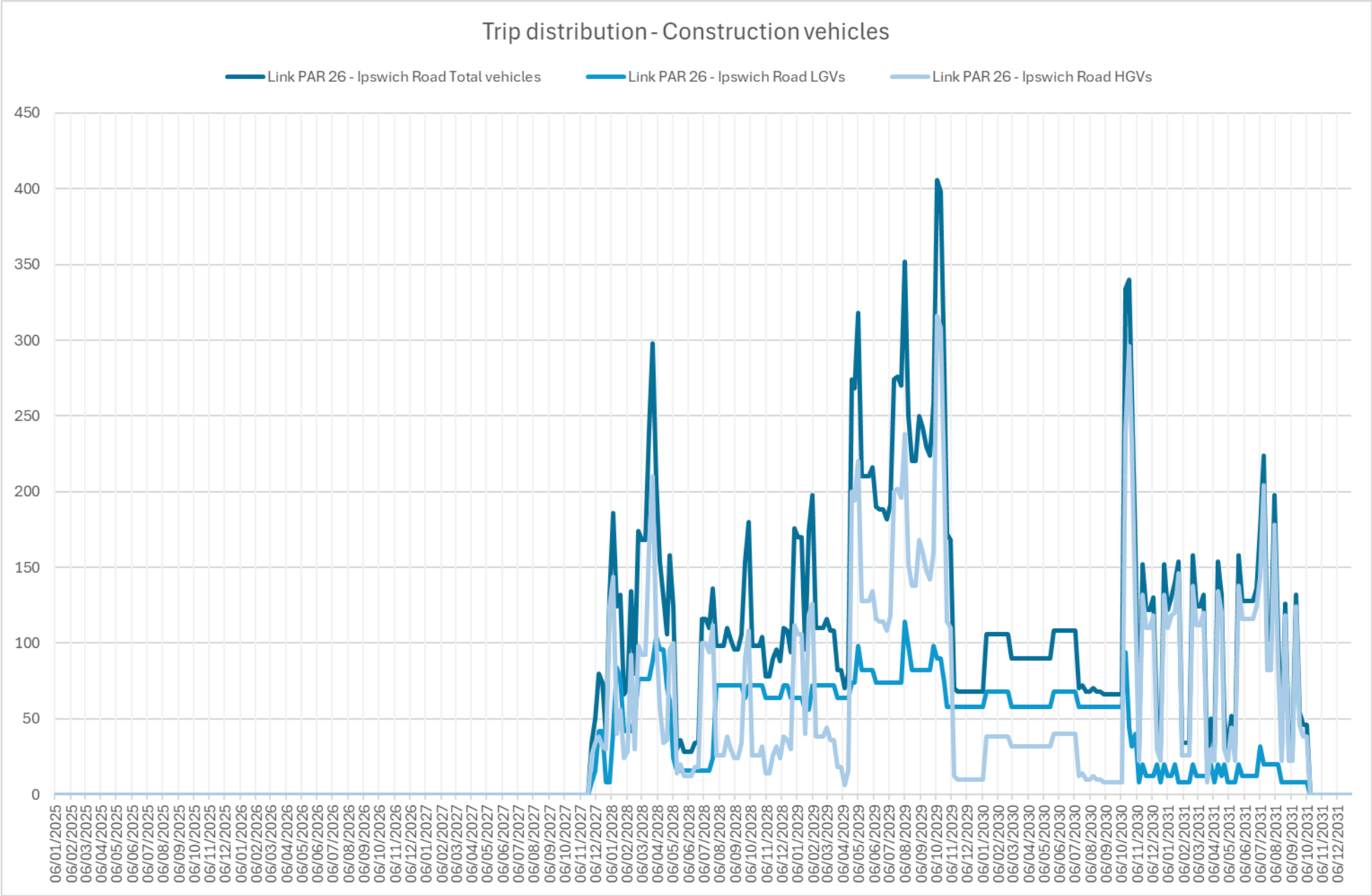
Image A16.4.26 Construction vehicles daily trip distribution of Ipswich Road (Link PAR 26)
