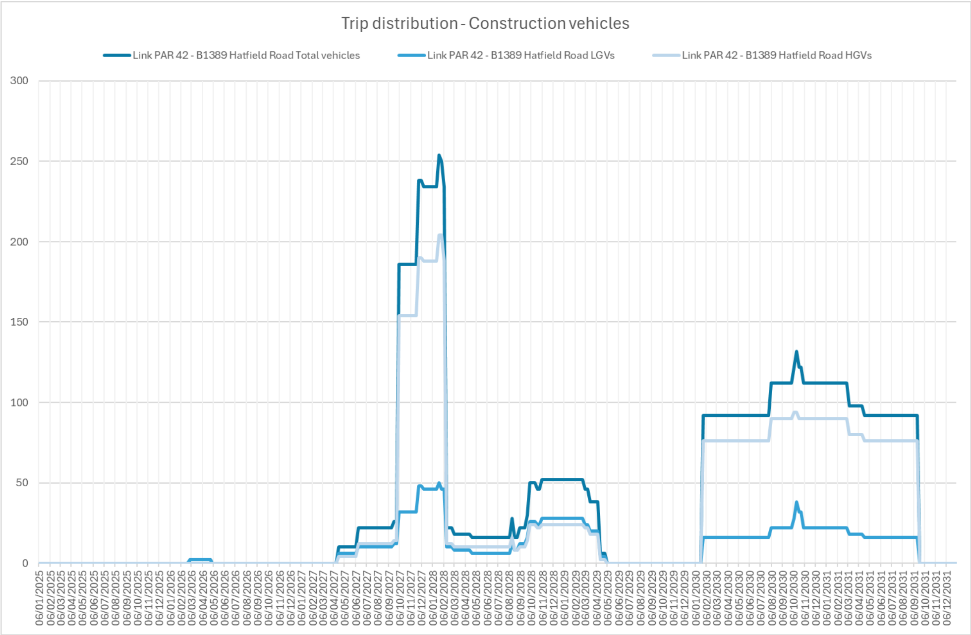
Image A16.4.42 Construction vehicles daily trip distribution of B1389 Hatfield Road (Link PAR 42)
