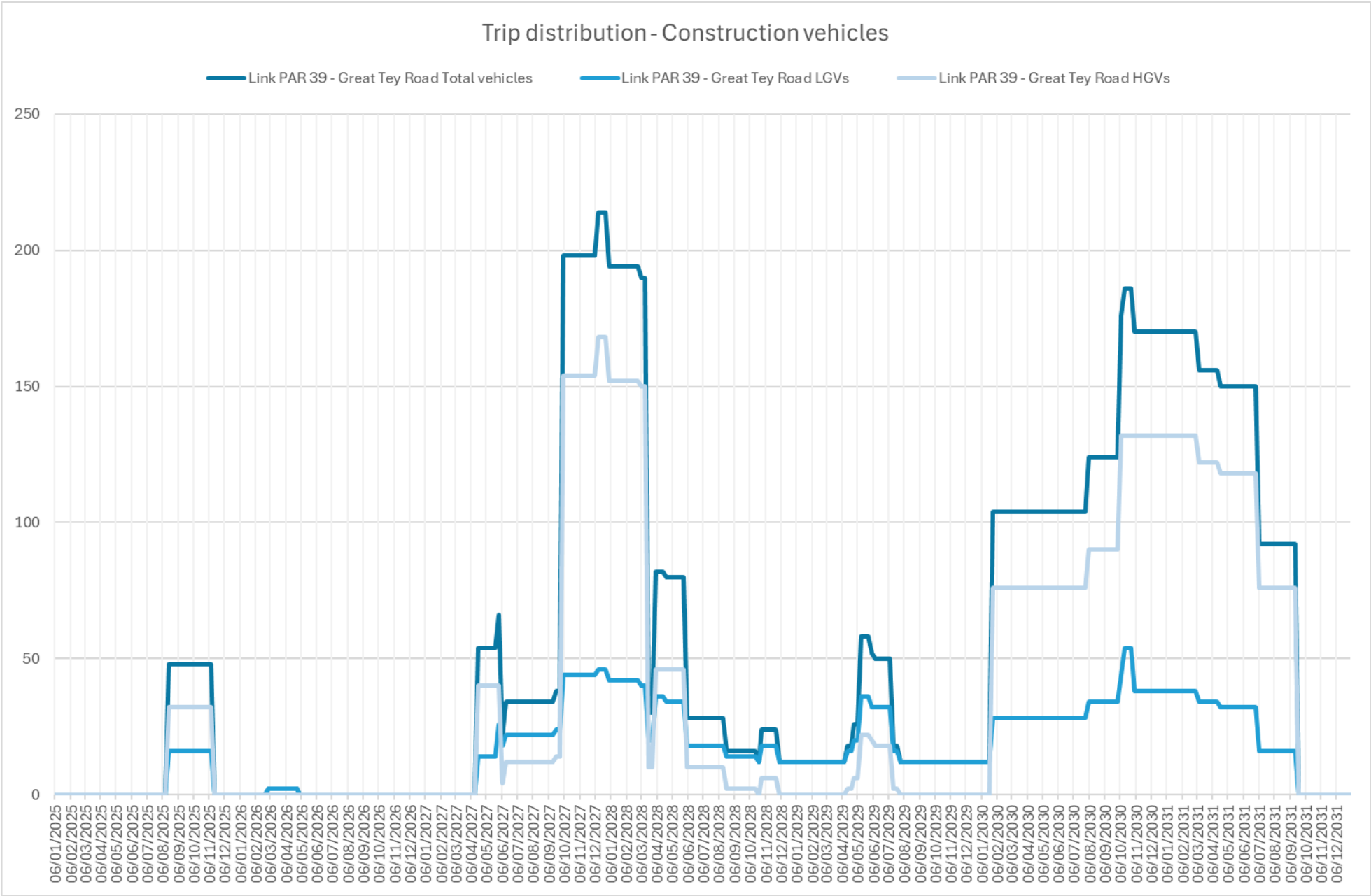
Image A16.4.39 Construction vehicles daily trip distribution of Great Tey Road (Link PAR 39)
